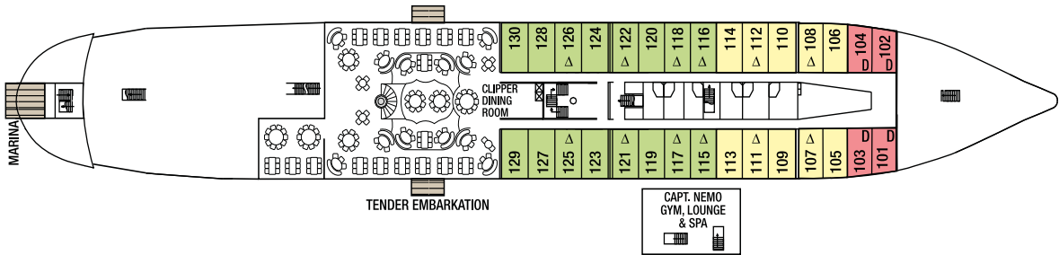
COMMODORE DECK
